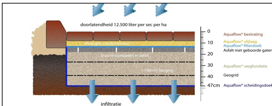
Aquaflow Industrial XL
